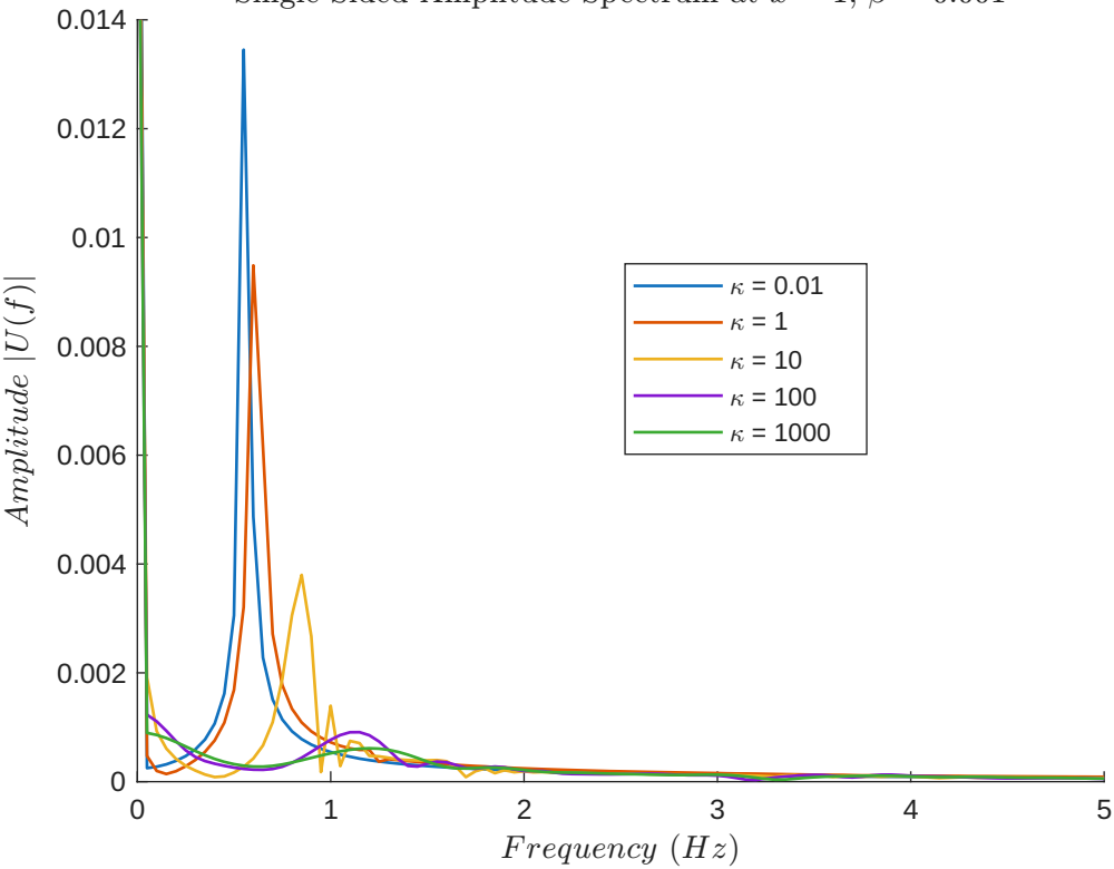
Single-Sided Amplitude Spectrum at x = 1 , \beta = 0.001
